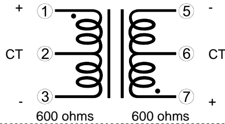
Schematics T1 (PC600/600)
