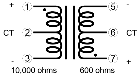
Schematics T1 (PC10k/600)
