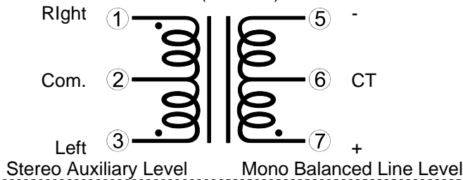
Schematics T1 (PC6400)
