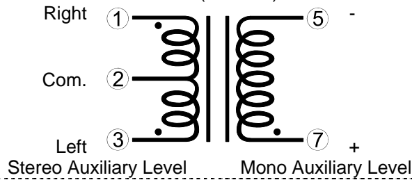
Schematics T1 (PC6410)
