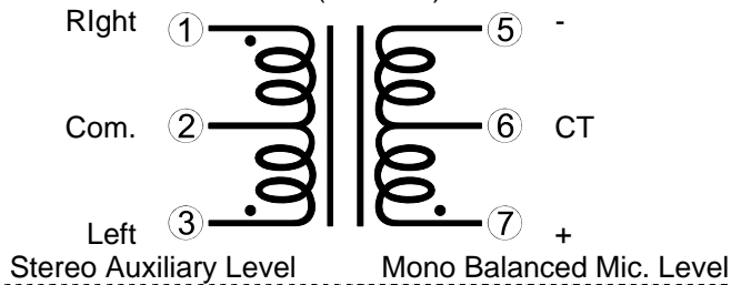
Schematics T1 (PC6415)
